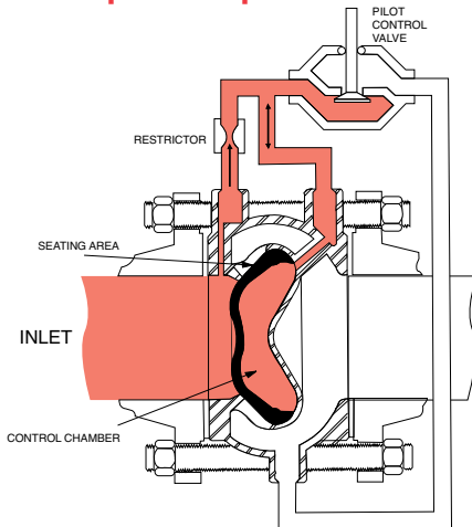
Model 100-42 Valve in Closed Position
