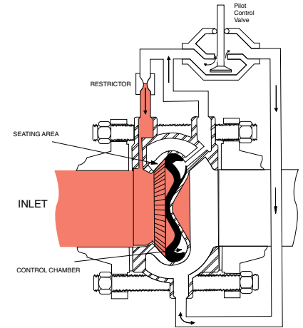
Model 100-42 Valve in Fully Open Position
