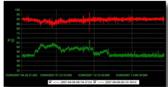
Pressure Management Tracker data output showing upstream and downstream pressure
