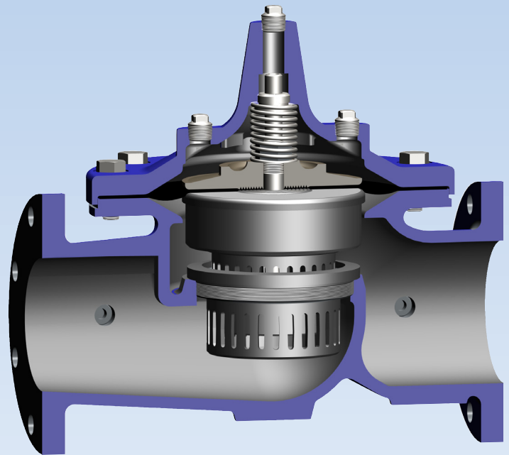
Main Valve with KO Anti-Cavitation Trim
